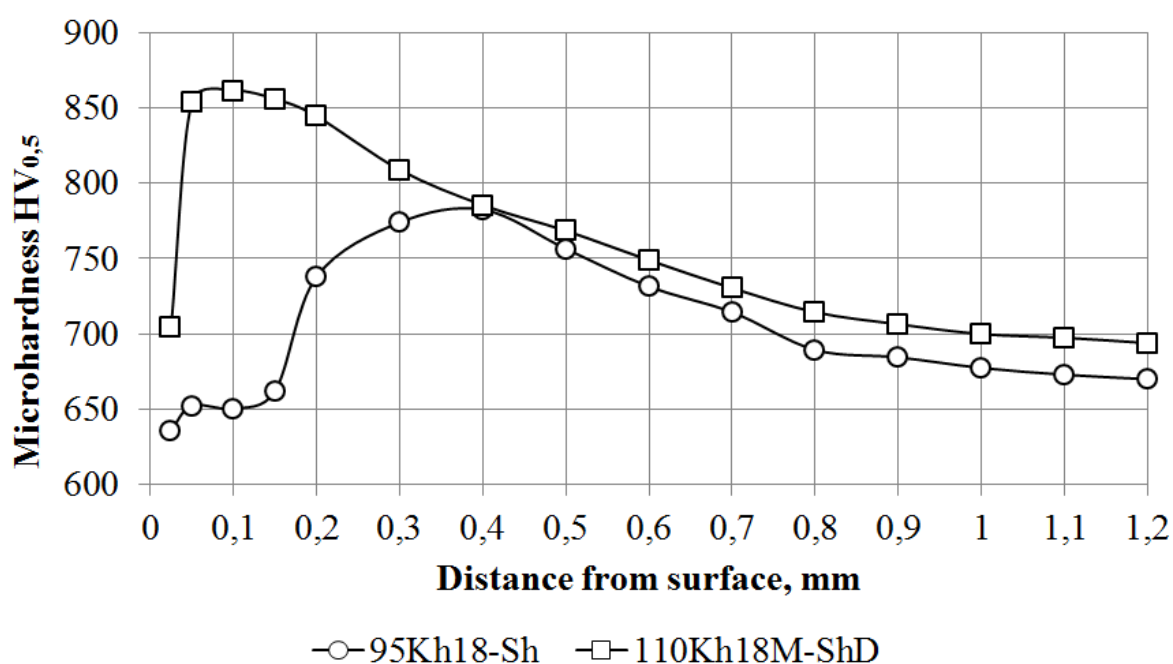
Figure 2. Distribution of microhardness of steels 95Kh18-Sh and 110Kh18M-ShD after vacuum nitrocarburizing
