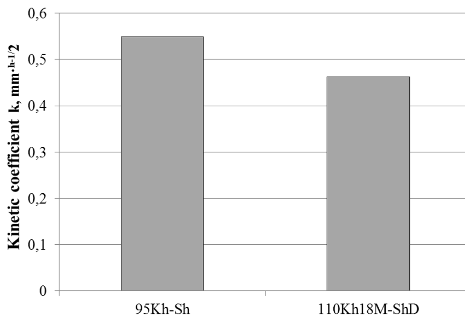
Figure 3. Kinetic coefficients of steels 95Kh18-Sh and 110Kh18M-ShD with simultaneous saturation with carbon and nitrogen
