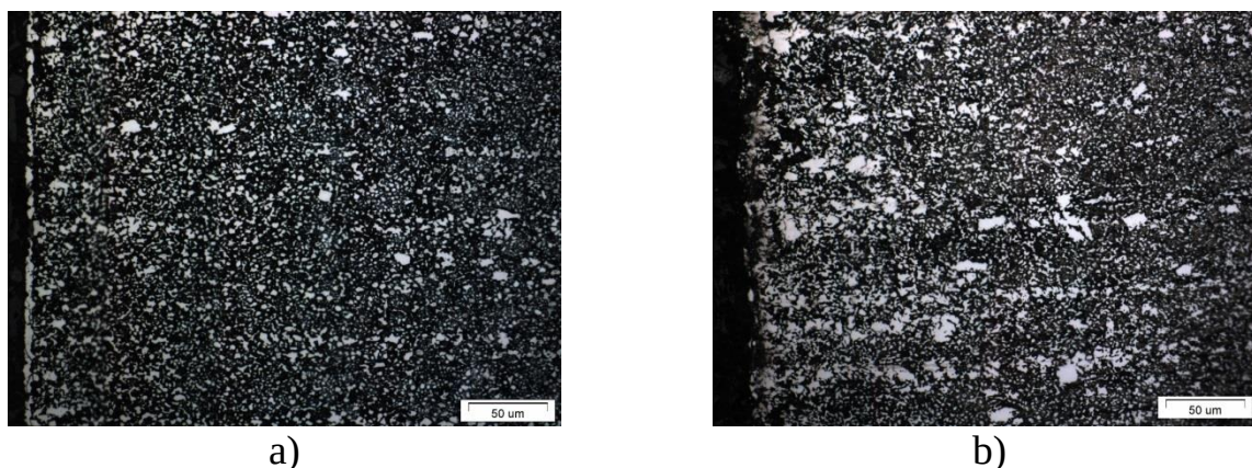
Figure 1. Microstructures of steels 95Kh18-Sh (a) and 110Kh18M-ShD after vacuum nitrocarburizing
